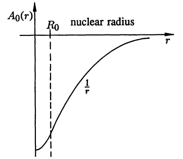
Fig. 1.3. The Coulomb potential of a negatively charged particle in the vicinity of the atomic nucleus
