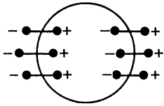
Illustration of the polarization in the surrounding of an electron under consideration
