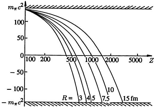
The energy of a \pi^- meson in the 1s state as a function of the nuclear charge Z . The radius was fixed at R = 3, 4, 5 fm, etc.
