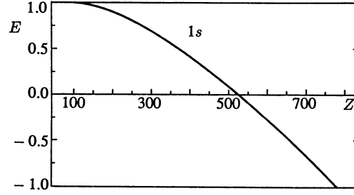
The energy eigenvalue of a 1s pion in an exponential potential as a function of the coupling strength parameter Z . The constant a characterizing the range of the potential is a = 1\lambda_\pi . The critical charge is Z_{\text{cr}} \simeq 778 . E is given in units of the rest-energy m_\pi c^2
