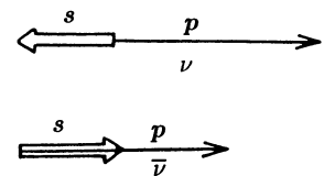
Fig. 14.1. The spin of the neutrino is always directed antiparallel to its direction of motion; the opposite is true for the antineutrino
