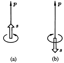
Fig. 2.2. Electrons with positive (a) and negative (b) helicity. The double arrow denotes spin. \odot and \ominus symbolize the two possible rotations of the electron
