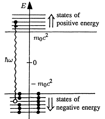
Fig. 12.4. The vacuum of the hole theory based on positrons as initial particles. Here a positron hole is an electron. As marked by the full circles (●) the states of negative energy are occupied with positrons
