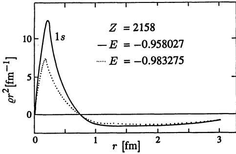
Fig. 1.4. The radial density \rho r^2 of a \pi meson in the 1s state of an exponential potential of the form V(r) = -Z\alpha \exp(-r/a) (see Exercise 1.15). The range parameter a of the potential is chosen to be a = 0.2\lambda , where \lambda_\pi = \hbar/m_\pi c is the Compton wavelength of the pion. The coupling strength is fixed by Z = 2158 . Such an extreme central charge is chosen to make various new features of the Klein-Gordon equation especially obvious. The energy eigenvalue of the 1s pion bound in this extremely short range and deep potential is E = -0.958027 measured in units of the rest energy m_\pi c^2 of the pion. It is evident that the charge density is not positive definite, and that antiparticles can also be bound in this potential. The radial density of antiparticle in the same potential is shown by the dashed line – the energy eigenvalue of a bound antiparticle is E = -0.983275 m_\pi c^2
