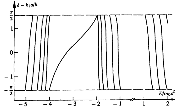
Fig. 9.6. The phase shifts of scattering states of a one-dimensional well of depth V_0 = -3m_0c^2 and with width a = 10\lambda_e as a function of energy E . The energy E is given in units of m_0c^2
