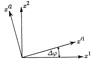
Fig. 3.4. An infinitesimal rotation of the coordinate system around the z axis
