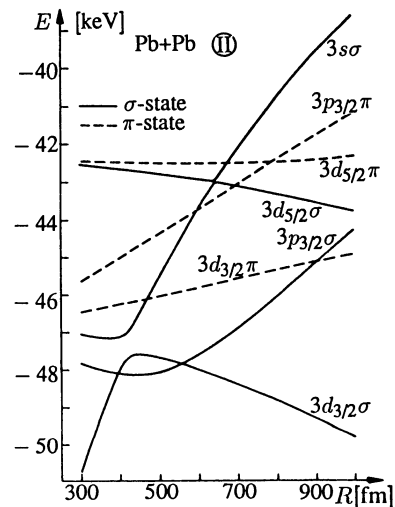
Fig. 10.4. Expanded sections from Fig. 10.3. The non-crossing of levels with at least one different quantum number is clearly noticeable
