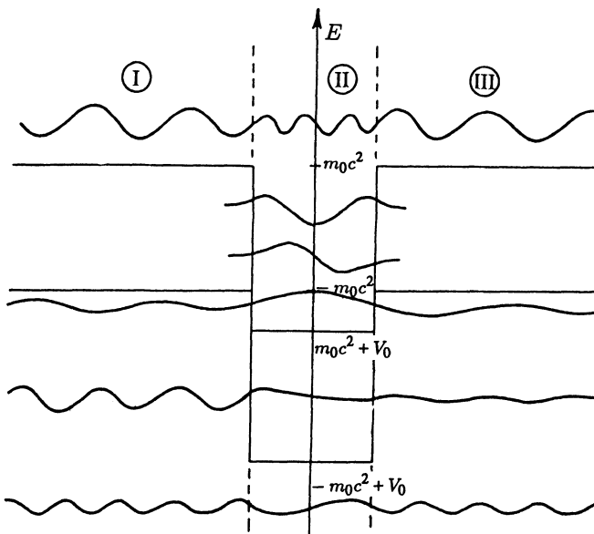
Fig. 9.2. The large component of some wave functions for different energies. In this case the depth is |V_0| > 2m_0c^2
