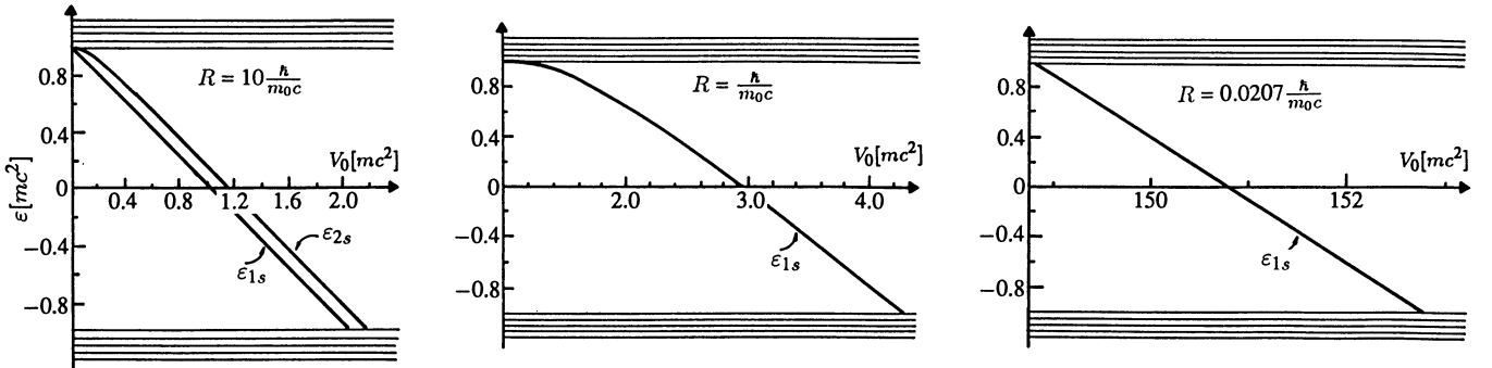
Fig. 9.11. 1s eigenvalues as a function of the potential strength for a spherical potential well. One example of the results for the 2s level are also shown
