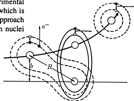
Fig. 10.1. Quasimolecular orbitals: The projectile ion moves along a curved trajectory. The individual atomic orbitals reappear when the colliding ions are separated enough (upper right). During the collision electrons (so-called \delta electrons – marked by \uparrow e^- ) and X rays \rightsquigarrow are emitted. The emission is caused by the varying molecular orbitals, which adjust themselves with respect to the varied internuclear separation
