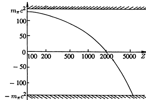
The energy of a \pi^- meson in the 1s state as a function of the nuclear charge Z . The radius of the nucleus is increased according to R = r_0 A^{1/3} where A = 2.5 Z is the number of nucleons in the nucleus
