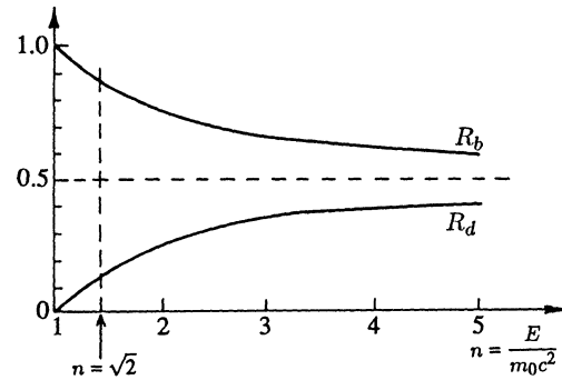
Relative intensities of partial waves of positive ( R_b ) and negative ( R_d ) energy is a Gaussian wave packet of width d
