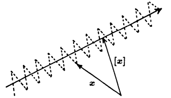
Fig. 2.4. Illustration of the Zitterbewegung in the forced one-particle picture. The location \mathbf{x} performs a Zitterbewegung around the mean (classical) trajectory [\mathbf{x}]
