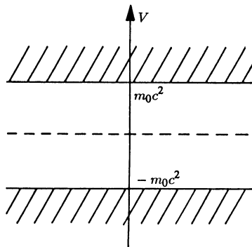
Energy levels of the free Dirac equation
