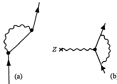
Fig. 9.17. (a) Self-energy diagram, (b) anomalous magnetic moment
