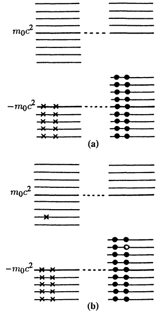
Fig. 12.6. (a) Illustration of the “symmetrized” vacuum state, consisting of states of negative energy filled with electrons (x) and positrons (•). (b) Illustration of a state with an electron in the second strongest bound level, which is indistinguishable from a positron hole in the second strongest bound positron level
