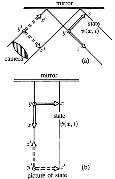
Fig. 12.7. Illustration of parity: The state \Psi(\mathbf{x}, t) is represented by a Dreibein (three unit vectors of a Cartesian coordinate system), which is filmed via the mirror. On the film the z axis appears (because of reflection) reversed. If the camera stood directly beside (in front of or under) the state, one would get the picture shown in b), with opposite z axis
