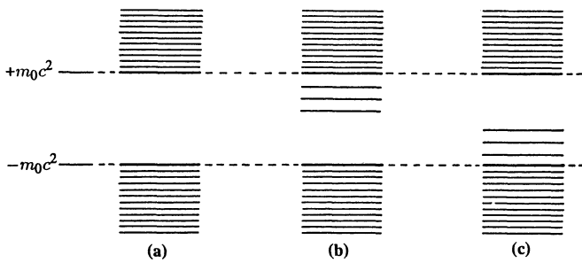
Fig. 12.5. Energy spectrum of a Dirac electron in an attractive Coulomb potential, a) free electron without potential, b) electron in an attractive potential -Ze^2/r , c) electron in a repulsive potential +Ze^2/r
