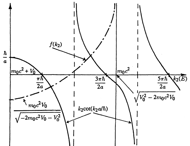
Fig. 9.3. The graphical solution of (19)
