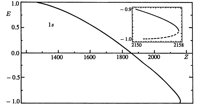
The same as in the foregoing figure for a = 0.2\lambda_\pi . The energy eigenvalues of bound antiparticles are also calculated. Z_{\text{cr}} \simeq 2158 . The insert in the figure shows \epsilon for the domain 2150 \leq Z \leq 2158 . The dashed line characterizes the energy of the antiparticle state
