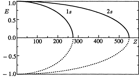
1s and 2s energies of the Klein-Gordon particles ( straight lines ) and antiparticles ( dashed lines ) in a scalar 1/r potential
