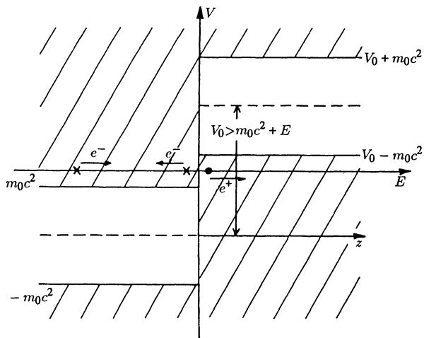
Energy continua of the Dirac equation at a potential barrier
