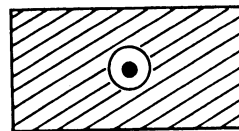
Nucleon surrounded by a sphere free of nuclear matter
