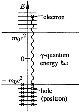
Fig. 12.3. A photon of energy \hbar\omega > 2m_0c^2 creates an electron-hole state. The hole is interpreted as a positron; hence the process is just e^- - e^+ pair creation
